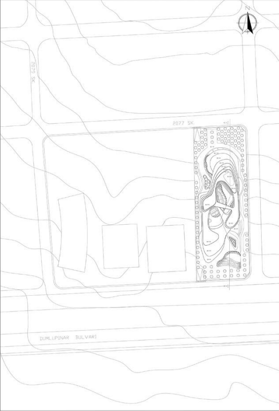
VAZİYET PLANI 1/500
